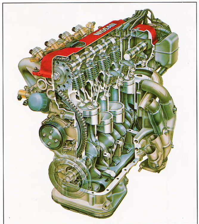
SR20DE Motor
