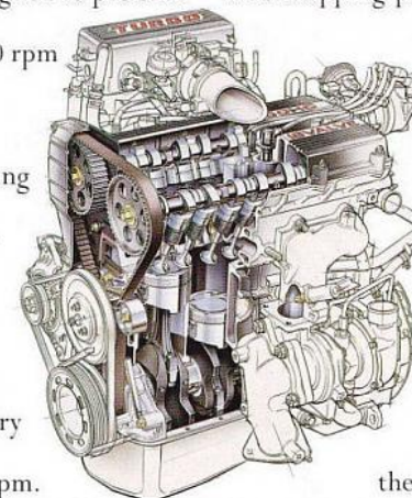
1.6 litre DOHC 16 valve, intercooled turbocharged engine.
