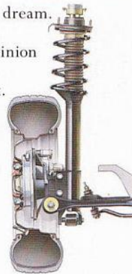
Independent sports suspension with front and rear stabilizers. (Manual only.)
