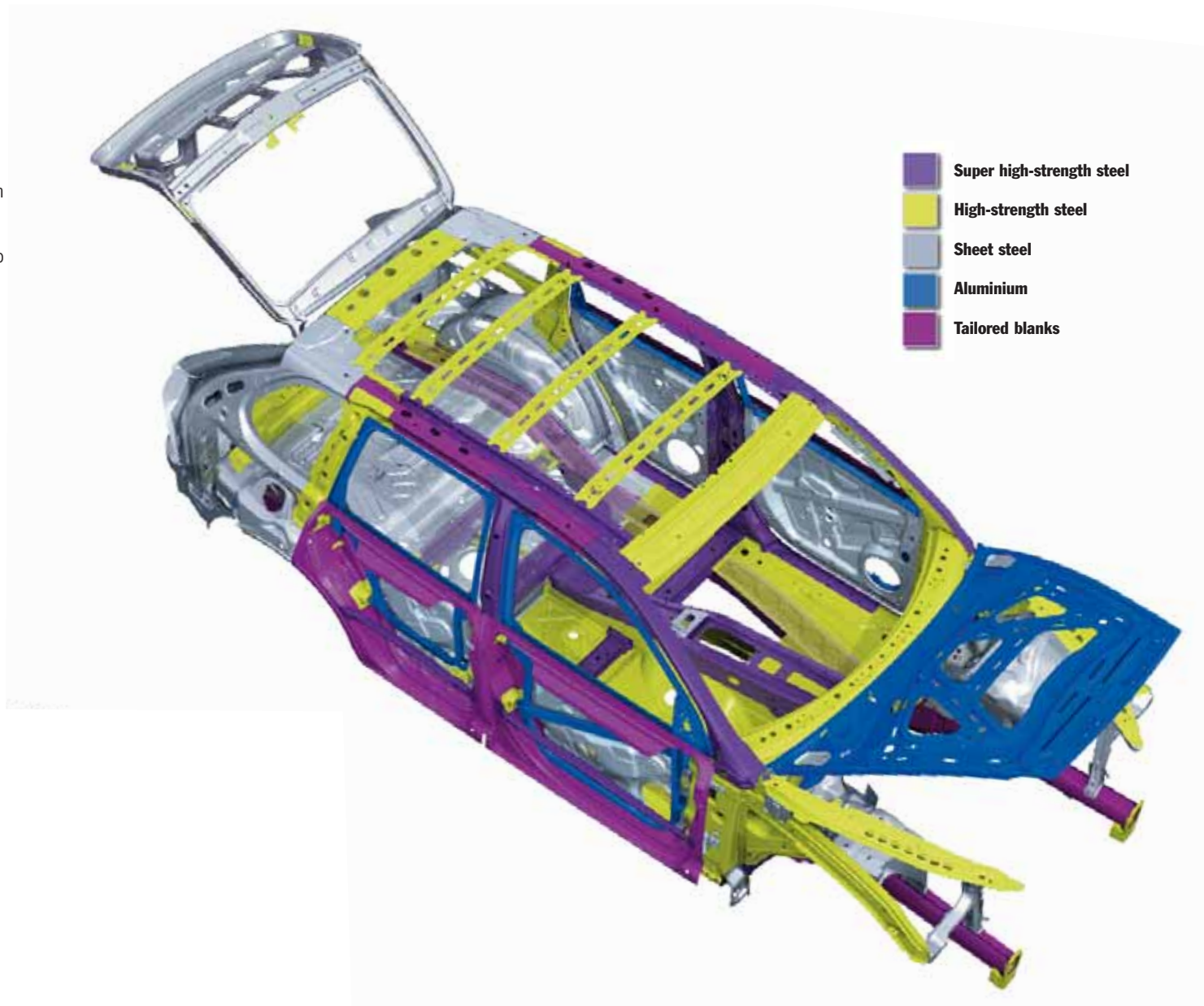
Passive safety: bodyshell
