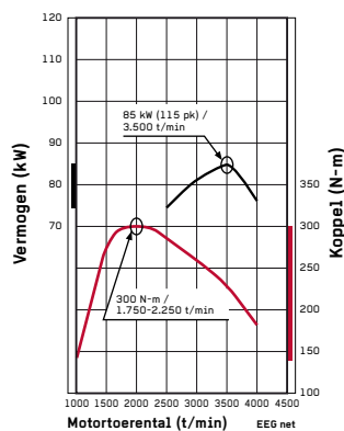
1.8-liter DI-D LP MIVEC
