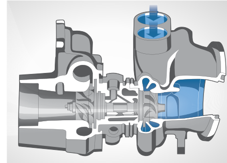
The TwinScroll Turbo in the BMW X1 xDrive28i has a modified turbine housing geometry. Two separate channels combining the exhaust from two cylinders do not merge until immediately before the turbine. The result: extremely spontaneous engine response and high performance.
