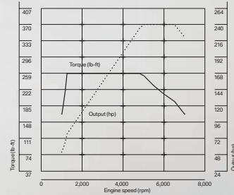
The 2.0-litre in-line four-cylinder engine of the BMW X1 xDrive28i provides maximum running smoothness all the way to an effortlessly attained maximum engine speed.
