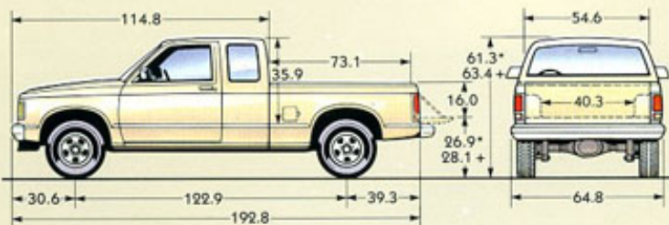
Club Coupe Pickup
