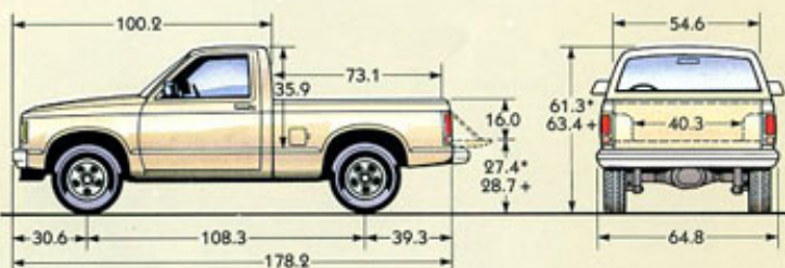
Short-Wheelbase Regular Cab Pickup
