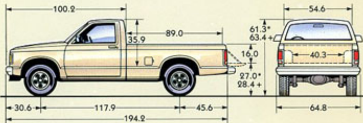
Long-Wheelbase Regular Cab Pickup
