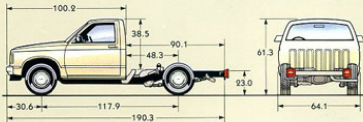
Cab & Chassis
