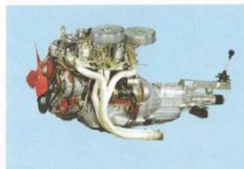
1600 GT high-performance engine
