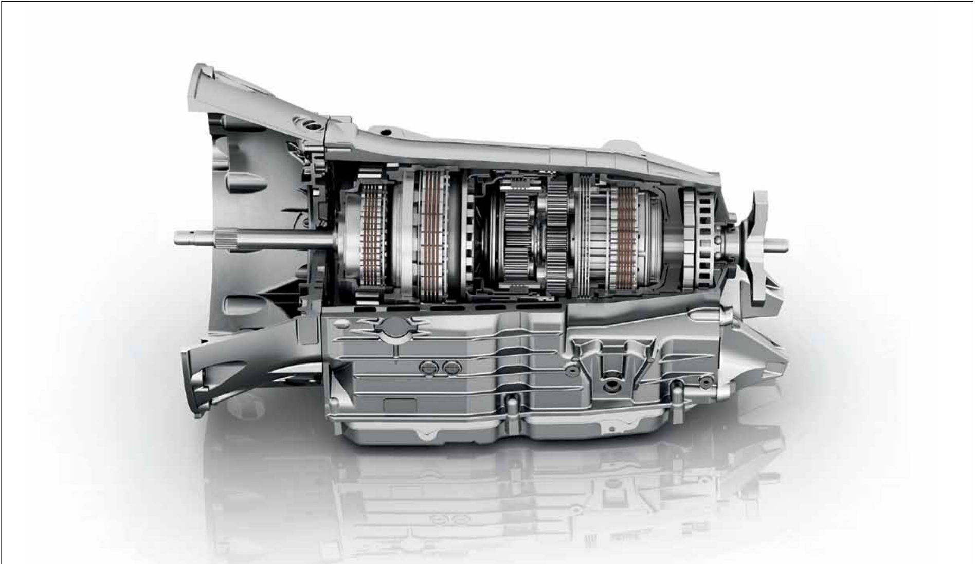
The 7G-TRONIC automatic transmission; one of over 18 million automatic transmissions produced in a period spanning more than 50 years.
