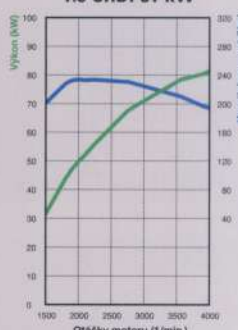
1.5 CRDi 81 kW
