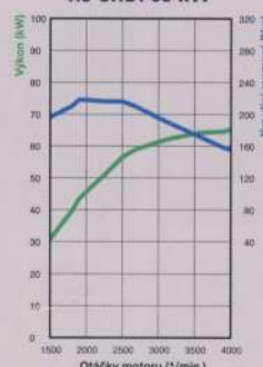
1.5 CRDi 65 kW
