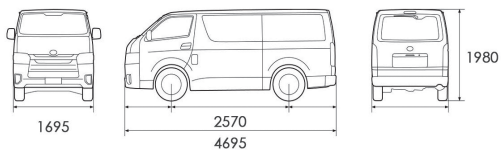
Standard Roof Van (Panel/Glass)
