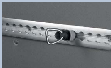
Movable lashing eyes. Purpose designed for the Opel Movano rail system. Made of steel with push-button locking mechanism.
