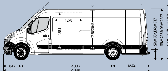
L4H2/H3 RWD (SRW/DRW)
