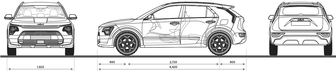
Dimensions Niro Hybride et Hybride Rechargeable (mm)
