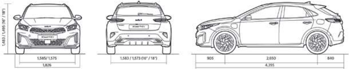
Dimensions Hybride Rechargeable (mm)
