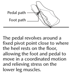
Organ-type accelerator pedal
