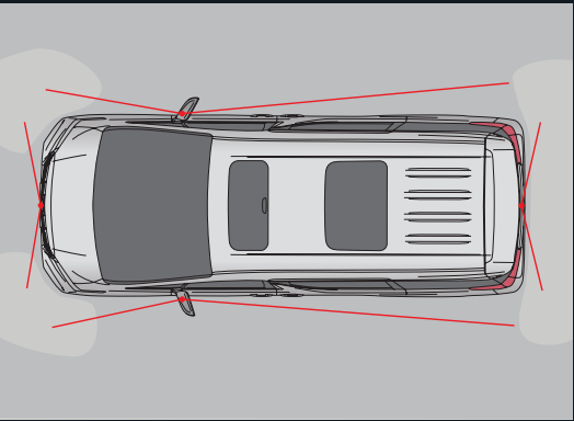
Surround Monitor Deliver 360 degree view from 4 cameras (front, left, right, rear) guides you during parking condition and tight road condition. (2.5 HV, 2.5 G & 3.5 Q Types)
