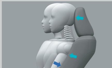
WIL Concept Front Seat In rear-end collision the occupant's upper body sink into the seatback with the back supported while headrest simultaneously support the head. (All Types)
