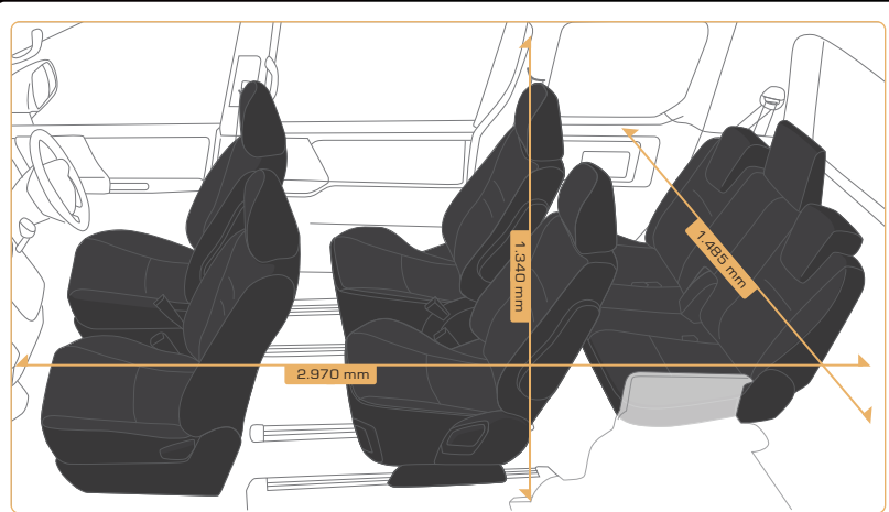
Interior Dimensions
