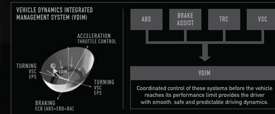
VDIM INTEGRATES ABS, EBD, BA, EPS, TRC & VSC SEAMLESSLY
