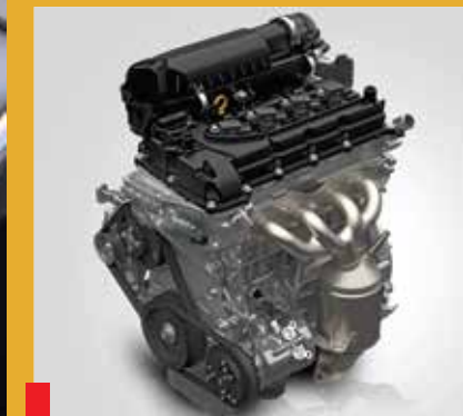
K-series Petrol Engine
