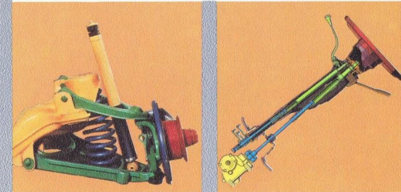
Individual wheel location and suspension
