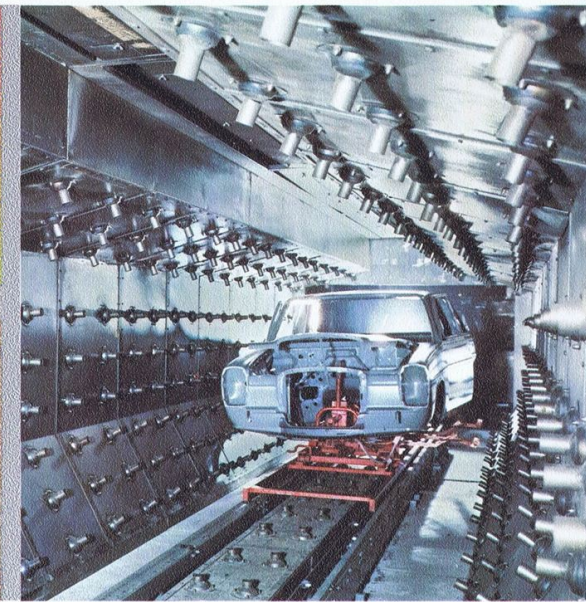
Cooling after paint annealing process
