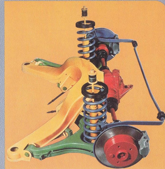
Diagonal swing axle
