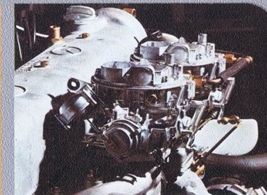
Two compound down-draft carburetors of the 250 C: 130 net b.h.p./DIN, 96 kW
