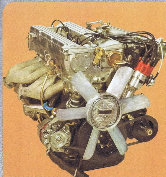
Twin-camshaft engine of the 280 C/280 CE: 160/185 net b.h.p./DIN, 118/136 kW
