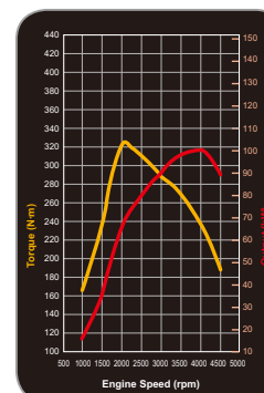
2.5-liter Intercooled Turbocharged DOHC DI-D Standard (100kW/4000rpm)
