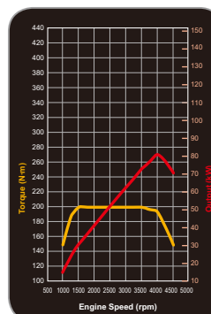
2.5-liter Turbocharged DOHC DI-D (81kW/4000rpm)
