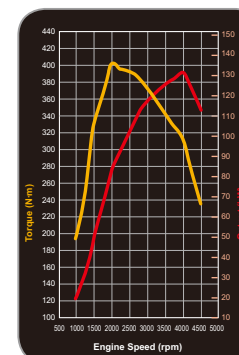
2.5-liter Intercooled Turbocharged DOHC DI-D High power (131kW/4000rpm)
