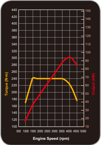
2.5-liter Intercooled Turbocharged DOHC DI-D (94kW/4000rpm)
