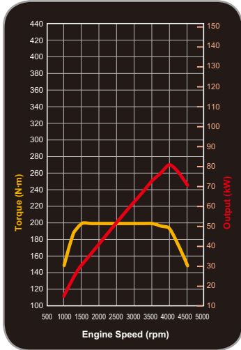
2.5-liter Turbocharged DOHC DI-D (81kW/4000rpm)
