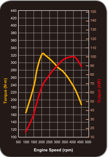
2.5-liter Intercooled Turbocharged DOHC DI-D Standard (100kW/4000rpm)
