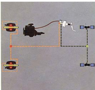
Dual-circuit brake system with brake booster.
