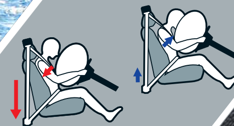
Seatbelt pretensioner and load limiter
