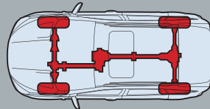
4WD low-gear mode
