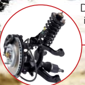
Double-wishbone suspension in front combined with 5-link suspension in the rear
