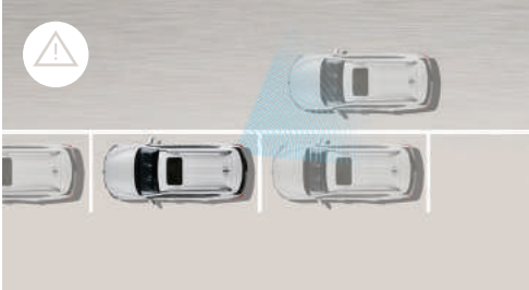
Safety Exit Warning (SEW) SEW uses rear corner radars to detect cars approaching from behind and warns passengers to look before exiting the vehicle.
