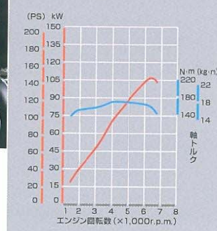
BEAMS 1ZZ-FE VVT-i Displacement: 1,754 cc Maximum Power: NET110kW (145PS) / 6,400r.p.m. Maximum Torque: NET171N·m (17.4kg) / 4,200r.p.m.
