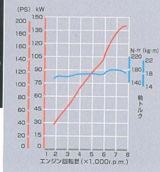
BEAMS 2ZZ-GE VVT-i Displacement: 1,795 cc Maximum Power: NET140kW (190PS) / 7,600r.p.m. Maximum Torque: NET180N·m (18.4kg·m) / 6,800r.p.m.
