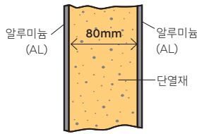
특수보온패널 (A80A) ※SIDE : A80A/FLOOR, ROOF FRONT : A80A
