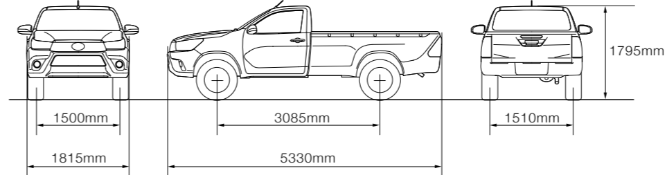
Single Cab/4WD (Long wheelbase)
