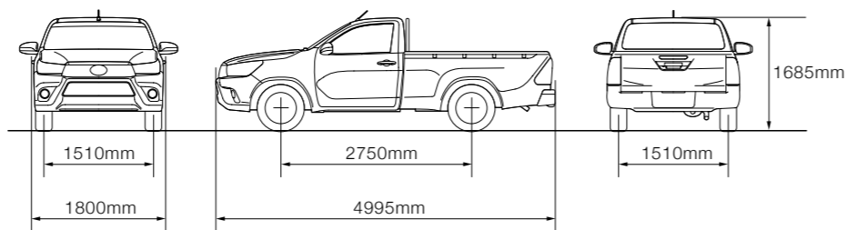
Single Cab/2WD (Short wheelbase)
