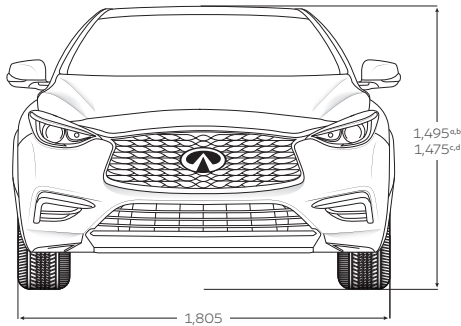
a 1.6t b 2.0t Premium c 2.0t Sport d 2.0t Sport AWD All dimensions are measured in mm.
