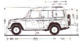
Dimensional Views Wagon (9-seater)
