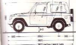
Dimensional Views Metal Top (4-seater)
