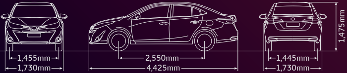
Note: Dimensions apply to the 1.5G variant only.
