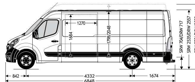
L4H2/H3 RWD (SRW/DRW)
