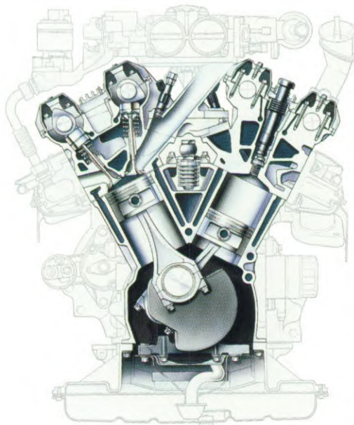
ECOTEC-3.0i- V6-24-kleppenmotor.
