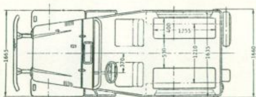
Lang chassis
