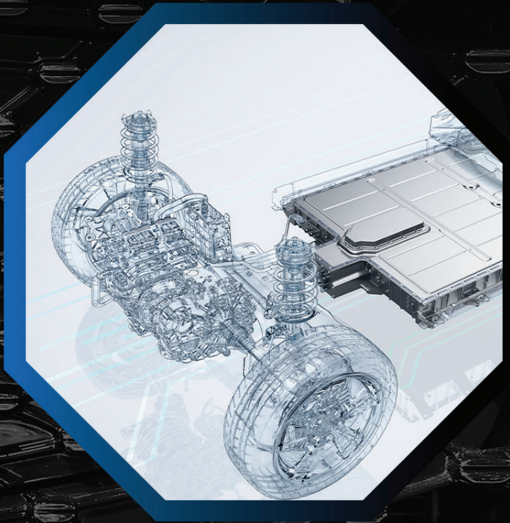
44.5kWh Water-cooled Lithium-ion Battery
