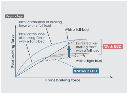
ELECTRONIC BRAKE DISTRIBUTION EFFICIENT AND EFFECTIVE BRAKING Working in tandem with ABS, it optimises the distribution of braking force between front and rear wheels.
