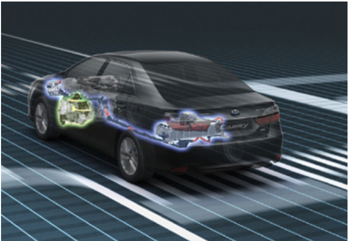
ZERO FUEL CONSUMPTION AND EMISSIONS When starting up from a stop , the electric motor can propel the Camry with electric power supplied solely by the hybrid battery. At this point, the Camry is almost silent, with zero petrol consumption and emission.
