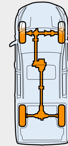
High range 4WD (4H)
