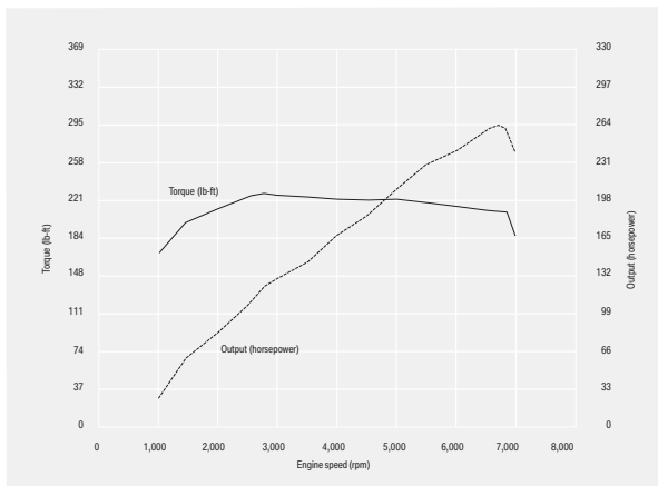
Torque-rich, free-revving and uncommonly smooth: the X3 s inline six eagerly revs to 7000 rpm, producing 260 horsepower at 6600 rpm and 225 lb-ft of torque at just 2750 rpm.
