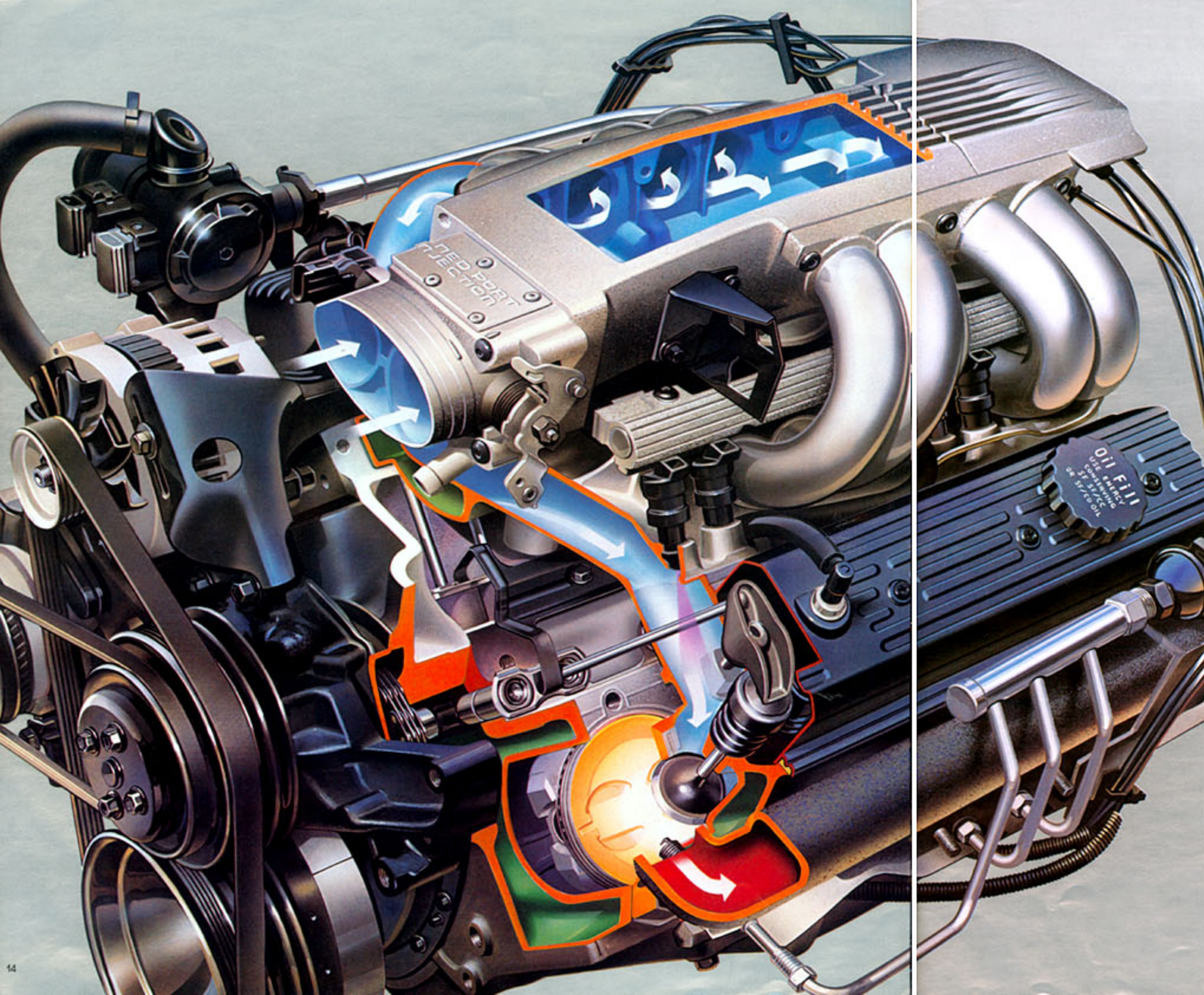
The 5.0L V8 with TPI, at left.
