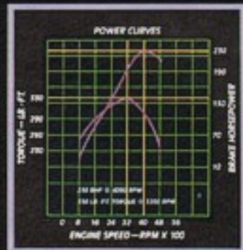
Horsepower-Torque Chart
