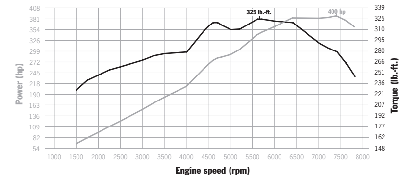
911 Carrera S: 325 lb.-ft. at 5600 rpm, 400 horsepower at 7400
