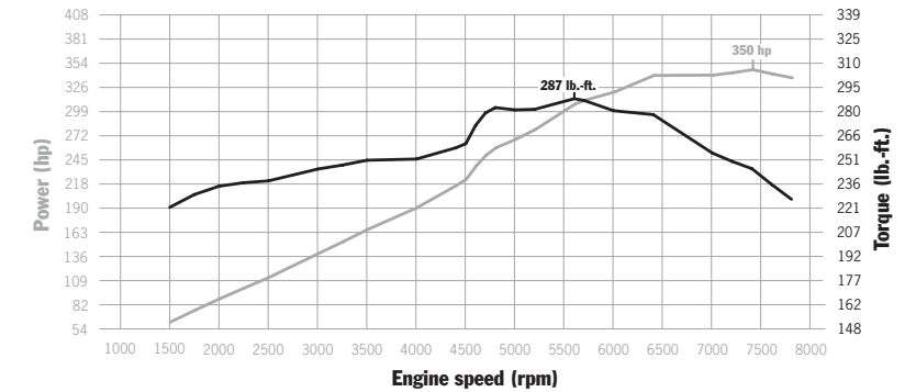
911 Carrera: 287 lb.-ft. at 5600 rpm, 350 horsepower at 7400 rpm
