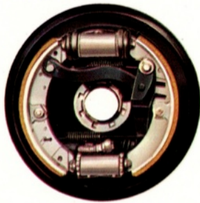
Rear Brake
