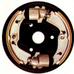
Front Brake
