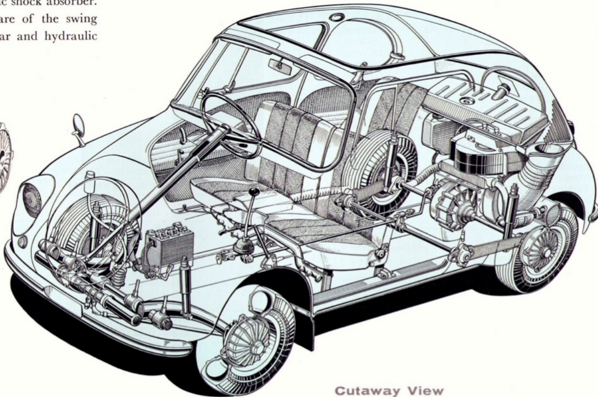
Cutaway View
