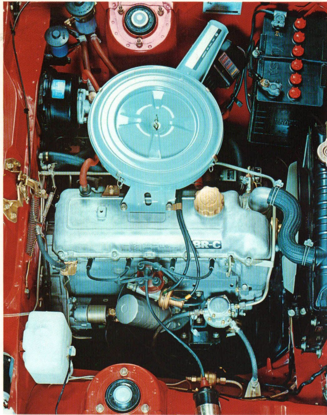
SOHC 4-in-line engine.
