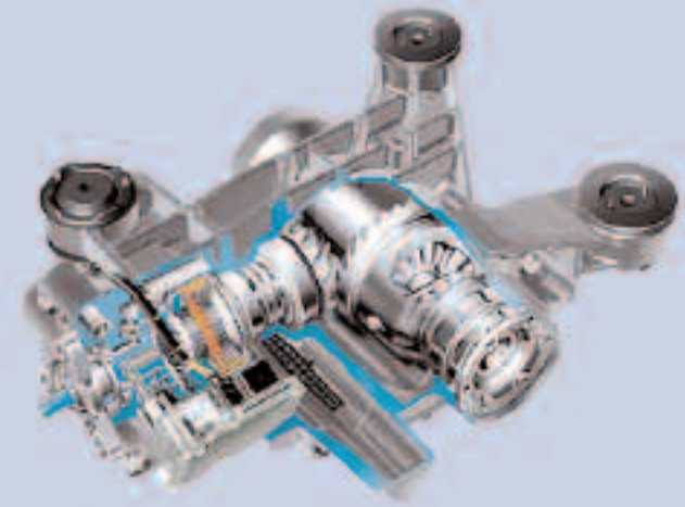
4MOTION all-wheel-drive system (detail)
