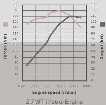
2.7 WT-i Petrol Engine
