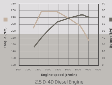
2.5 D-4D Diesel Engine
